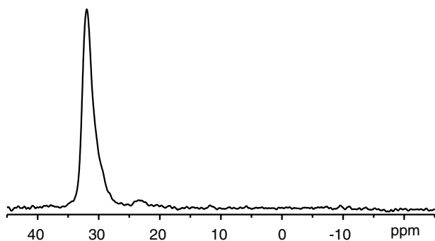
Fig. 2. The quality of the aligned membrane samples was checked by ^{31}\text{P} NMR. The example shown for (\text{CF}_3)_2 -GS/K in DMPC confirms nearly 100% alignment (intensity at \sim 30 ppm), and almost no unoriented powder contribution (intensity at \sim -10 ppm).
