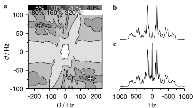
Fig. 3. The fitting procedure was validated using the model compound (\text{CF}_3)_2 -PhA carrying two \text{CF}_3 -groups (see Fig. 1b). Simulated and experimental spectra were compared on the basis of root mean square deviations (rmsd) by systematically varying the intra - and inter - \text{CF}_3 couplings D and d (a). The best fit (b) found this way for D = +(-)163 \text{ Hz} and d = -(+)72 \text{ Hz} reproduces the experimental spectrum (c) in all detail. (The percentages for the contour levels refer to the deviation from the global rmsd minimum, which are marked by +.)
